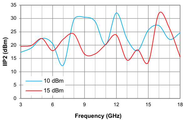
Input IP 2 , F IF1 = 34 MHz, F IF2 = 35 MHz
