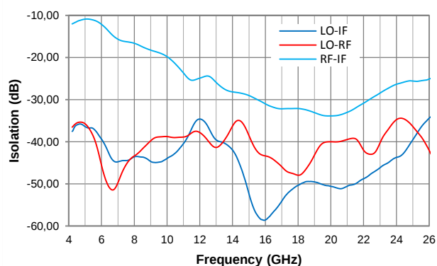
Isolation, PLO = 15 dBm
