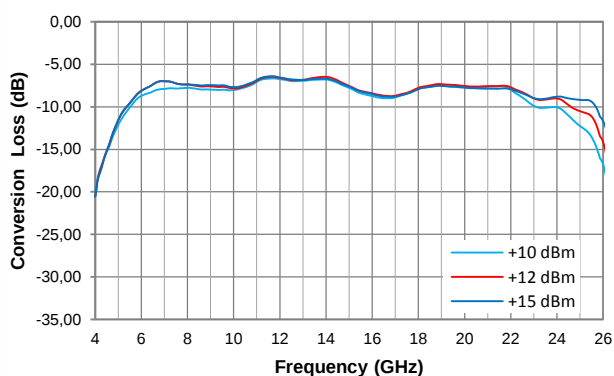
Conversion Loss
