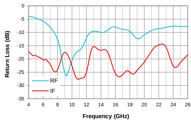
Return Loss
