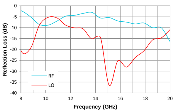
Reflection Loss
