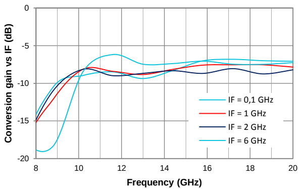
Conversion gain vs. IF
