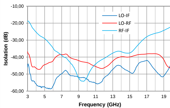
Isolation (config. B), PLO = 15 dBm
