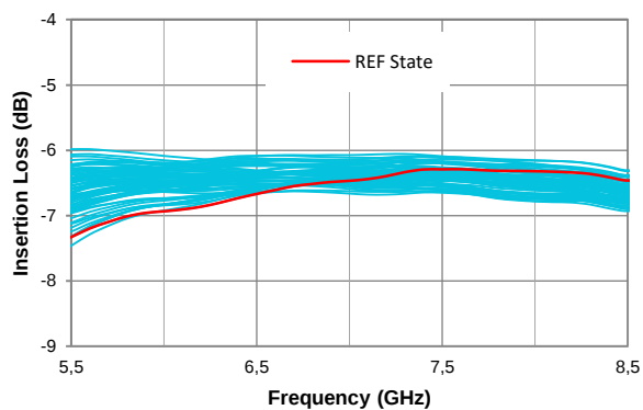
Insertion Loss
